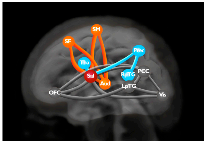
Fig. 1. COI. Edges represent lower functional connectivity between components in preterm controls than in full-term newborns. Node localization is based on the local maxima of the z-score within each network. Orange: module M1; blue: module M2; black: module M3. Sal, salience network; Aud, auditory cortex; Tha, thalamus; RptTG, right posterior temporal gyrus; Vis, visual cortex; LpTG, left posterior temporal gyrus.
